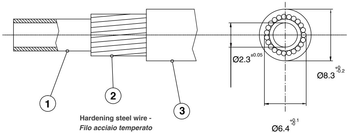
Inner liner - Tubetto
